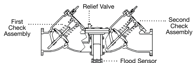
909RPDA with flood sensor
